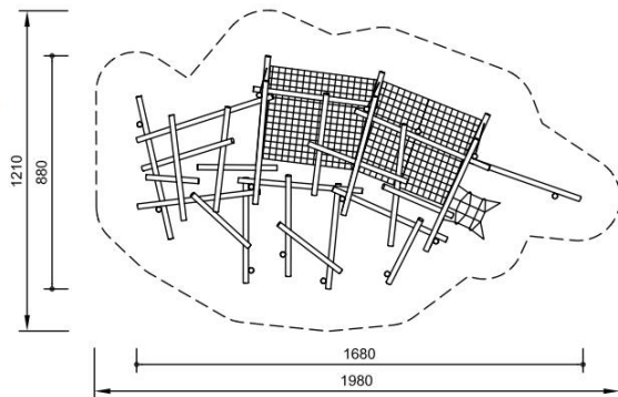
scale 1:200 dimensions in cm
