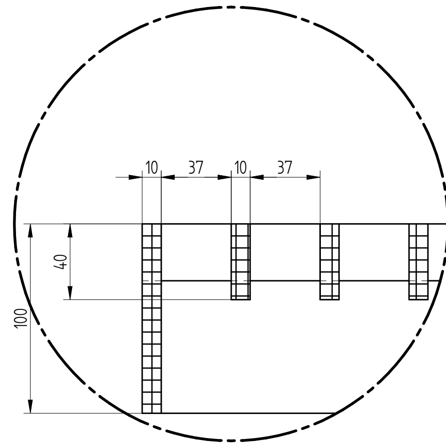
DETAIL B
